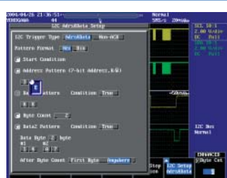
I 2 C bus trigger setup menu
